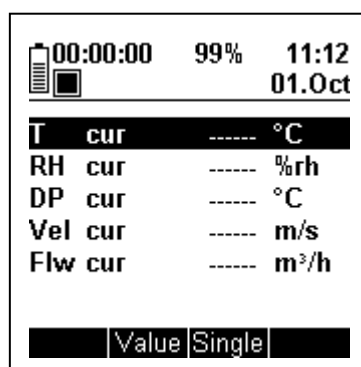
Picture 3.2: Normal mode – microclimatic probe connected, measurements stopped
