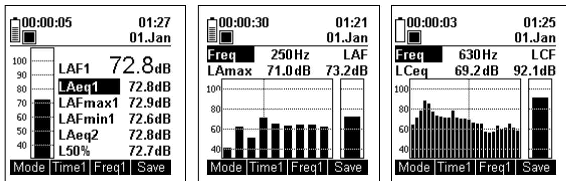
Picture 3.9 Three sound measurement submodes
